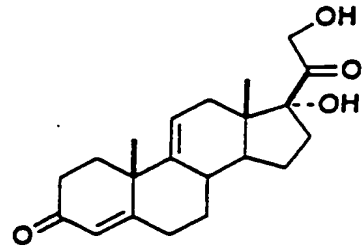
4,9(11)-Pregnadien-17a,21-diol-3,20-dione
